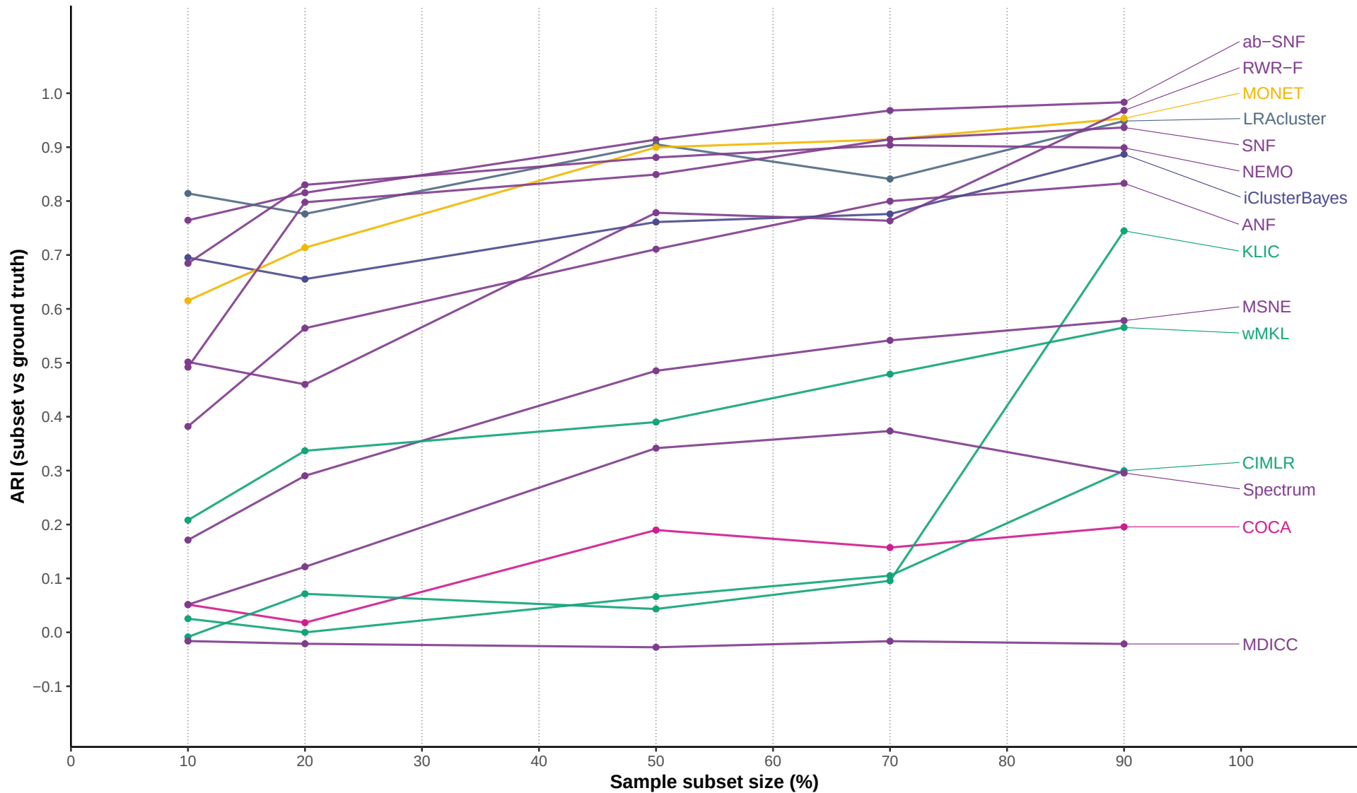
Agreement with ground-truth clustering under sample perturbations
