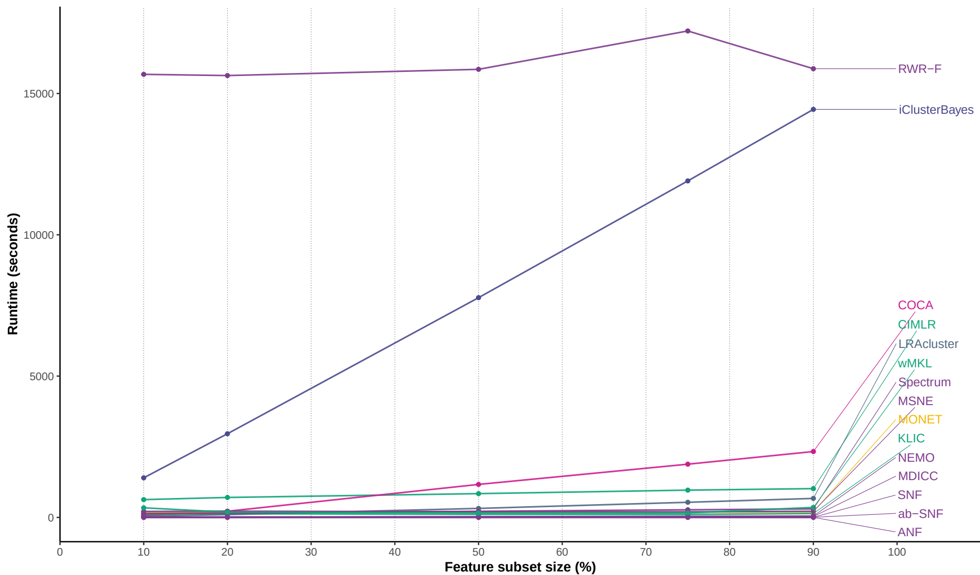
Runtime under feature perturbations
