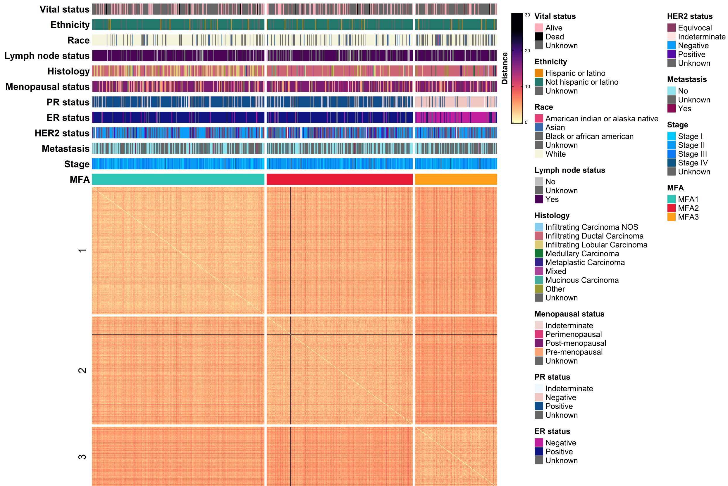
MFA embeddings distance matrix
