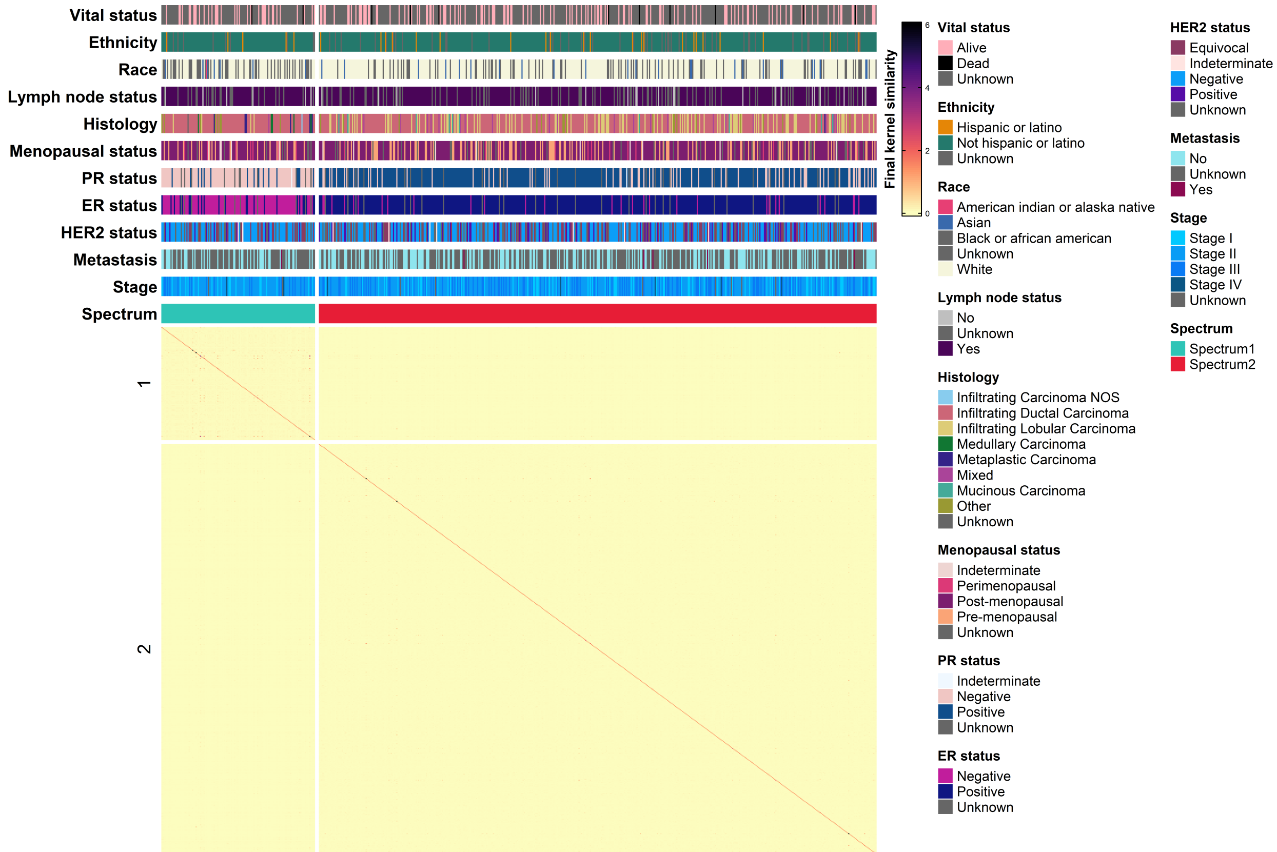
Final Spectrum similarity (S matrix) heatmap
