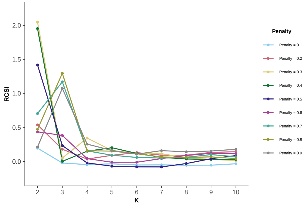
RCSI vs. number of clusters K for different Penalty values
