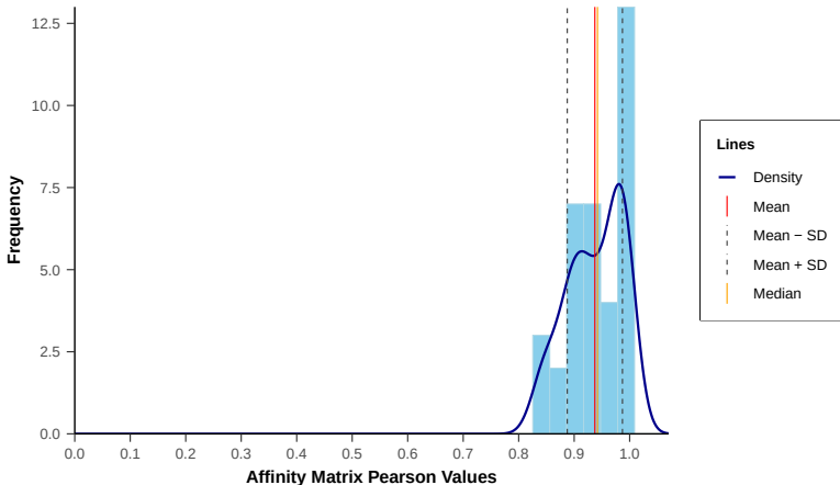
Histogram of Pearson values between affinity matrices for varying kNN_p values
