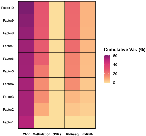
Cumulative Variance Explained Plot: 10 Factors
