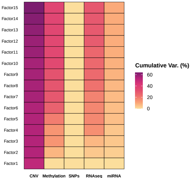
Cumulative Variance Explained Plot: 15 Factors
