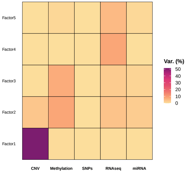
Variance Explained Plot: 5 Factors
