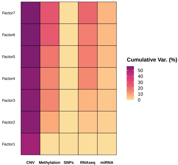
Cumulative Variance Explained Plot: 7 Factors
