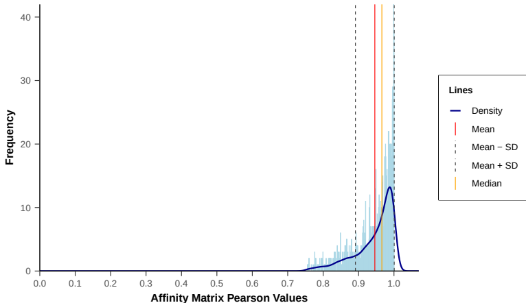
Histogram of Pearson values between affinity matrices for varying NN and \sigma values
