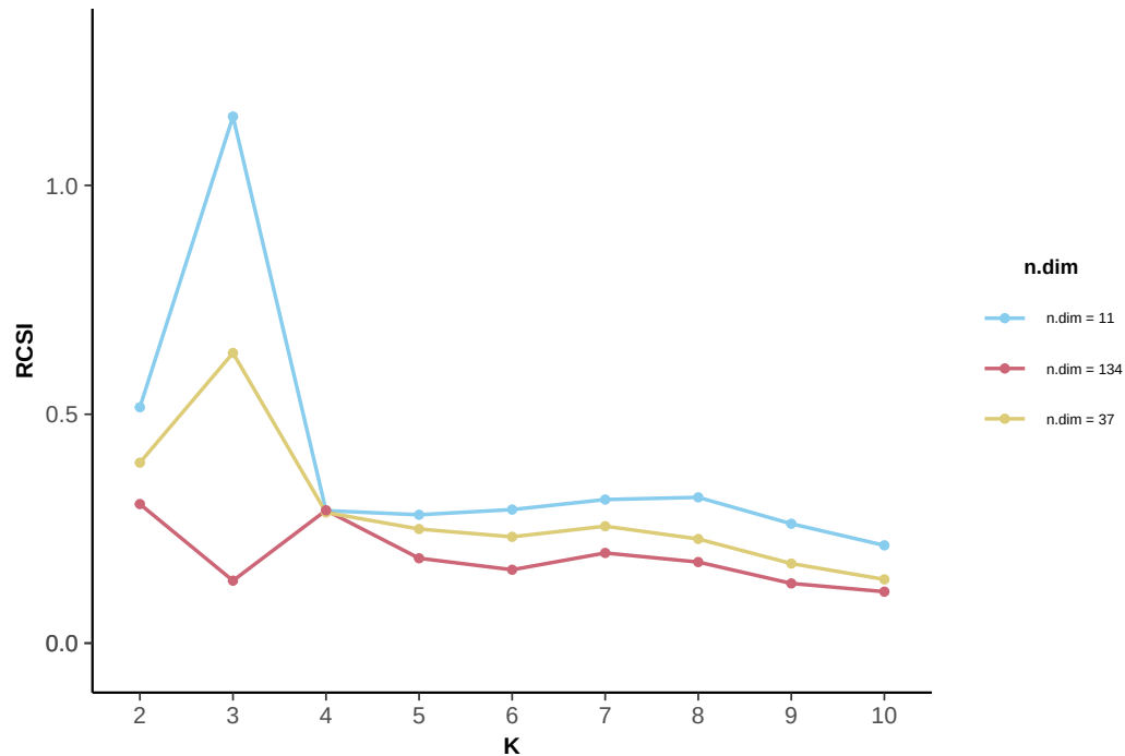
RCSI vs. number of clusters K for different n.dim values
