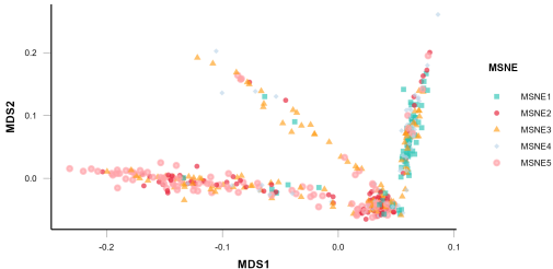
Multidimensional scaling: SNPs
