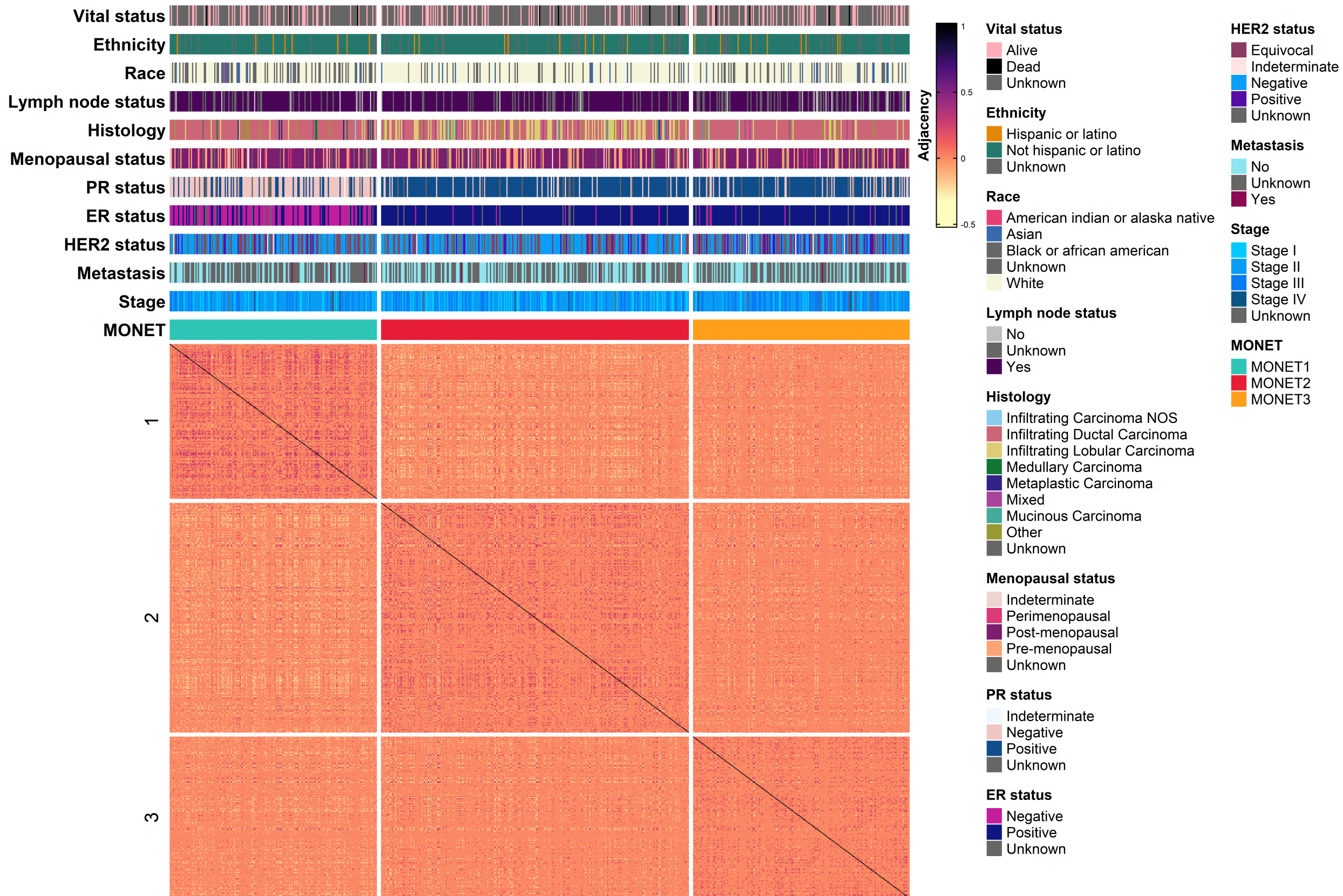
RNAseq adjacency heatmap
