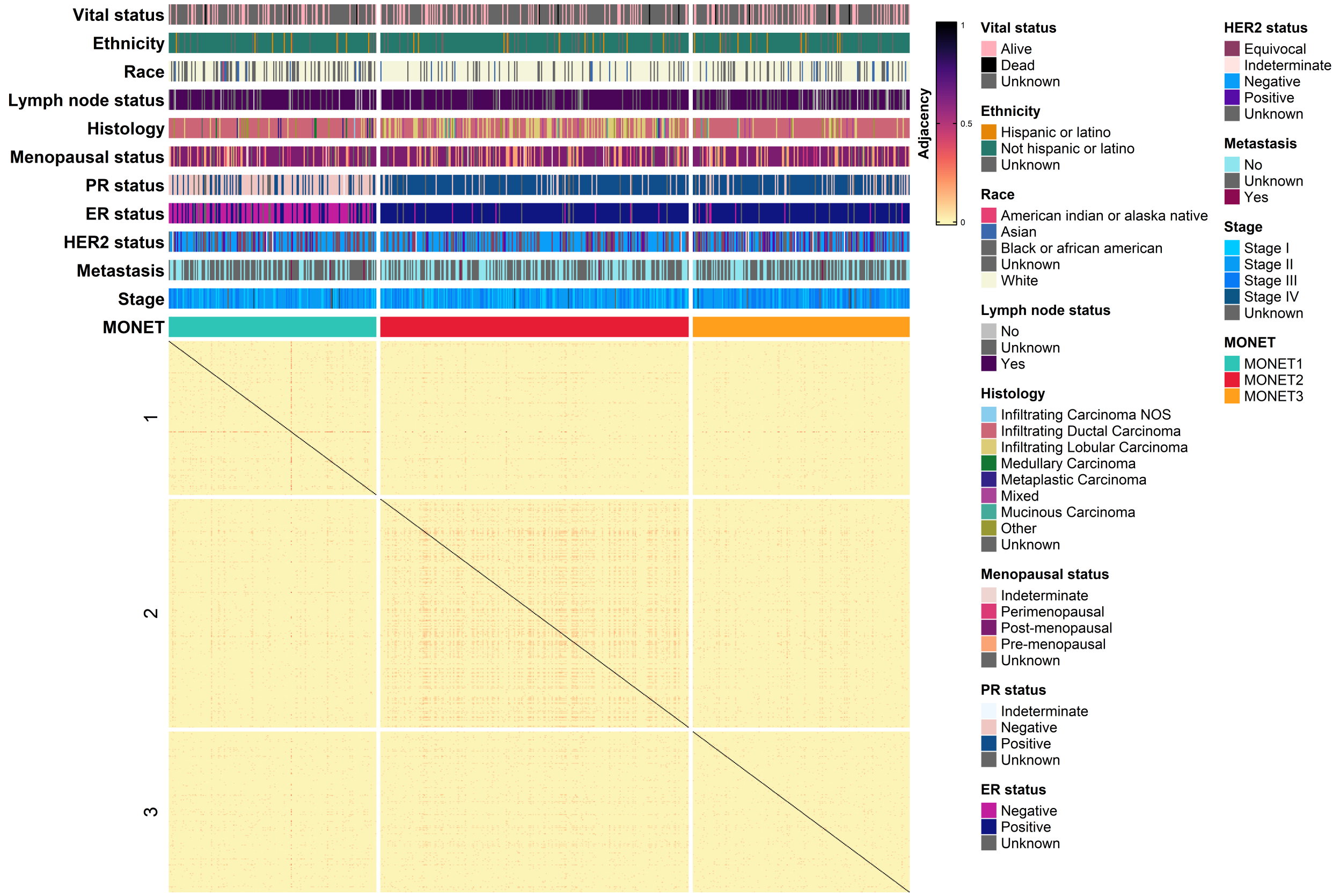
SNPs adjacency heatmap
