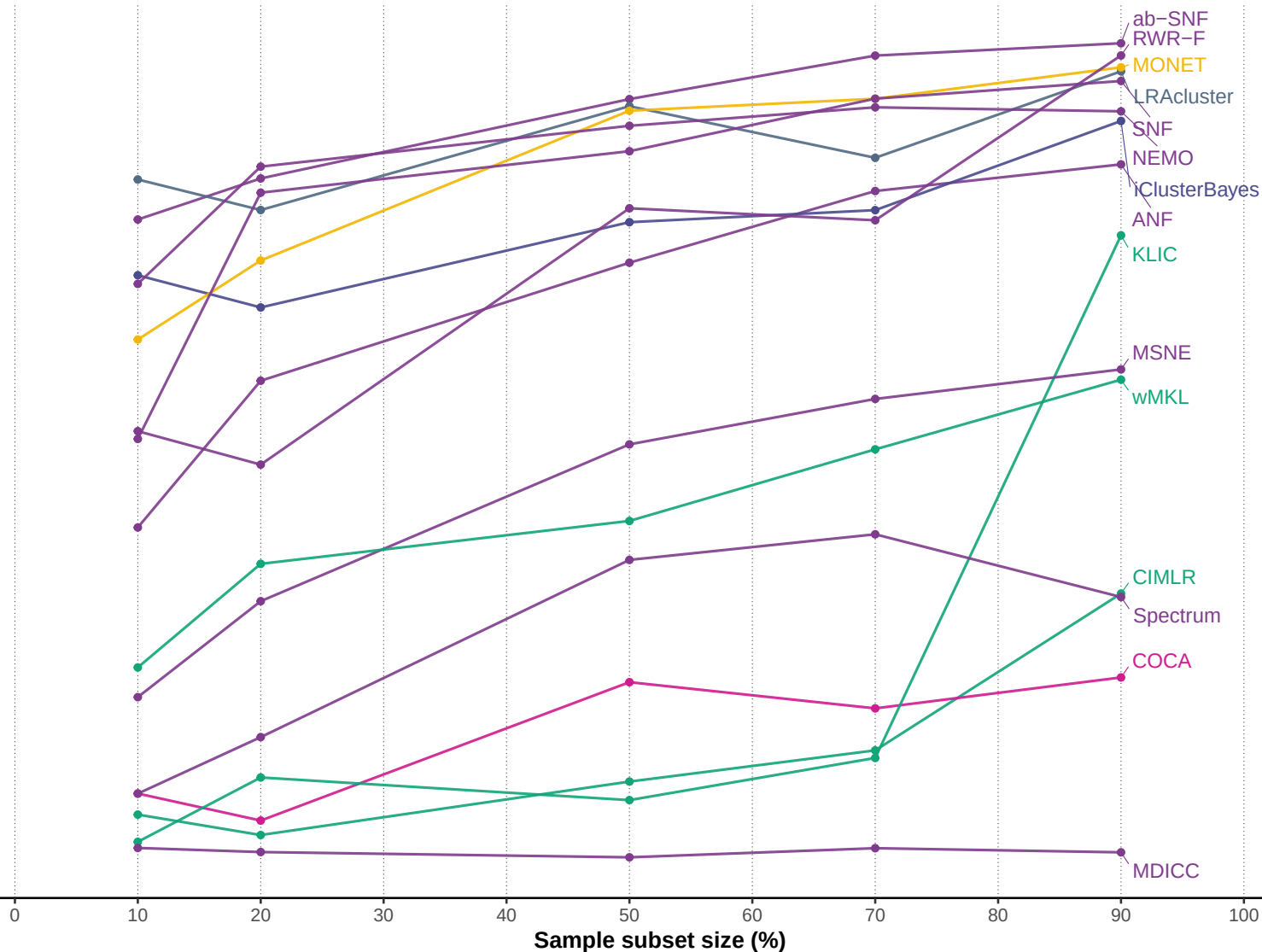
Agreement with ground-truth clustering under sample perturbations
