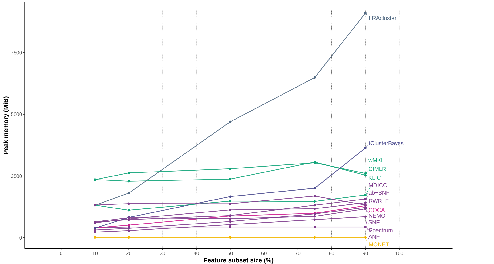
Peak memory under feature perturbations
