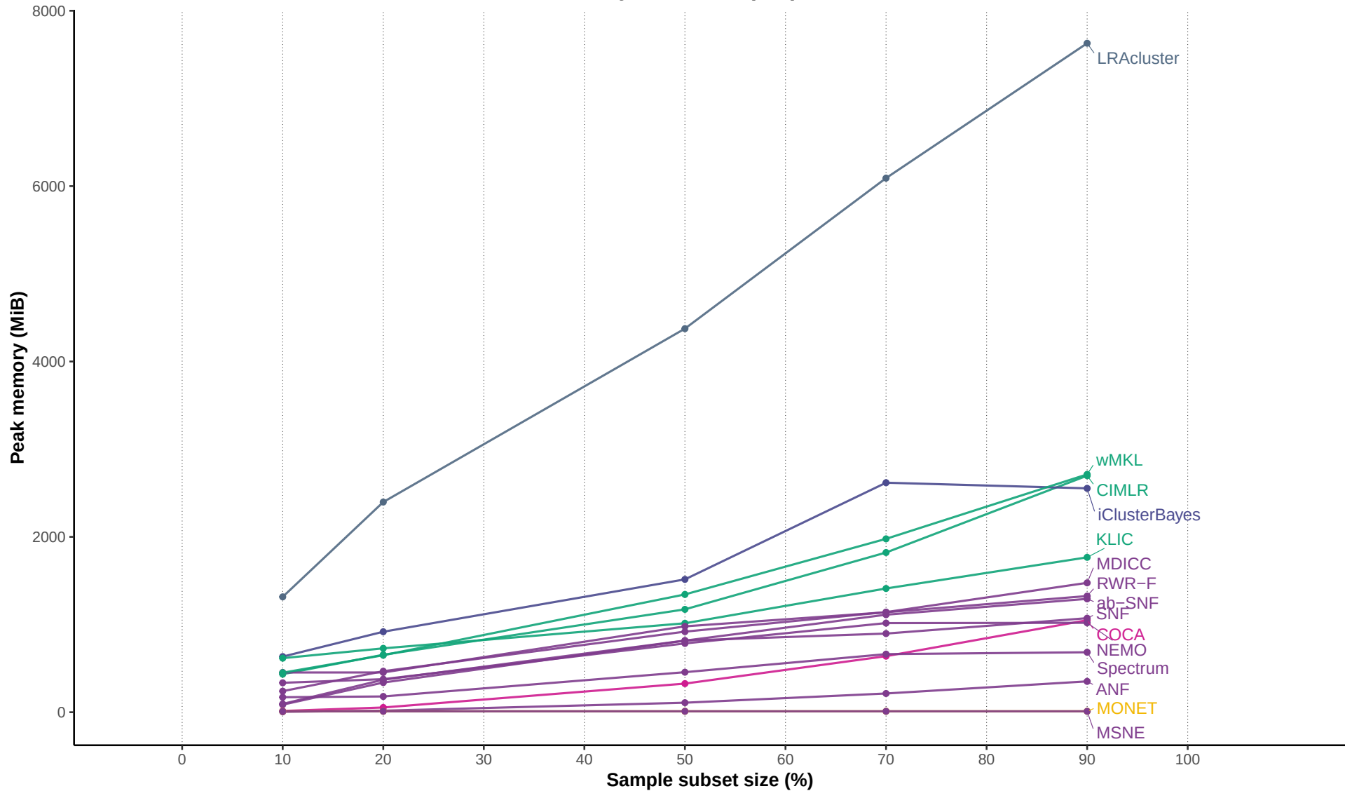
Peak memory under sample perturbations
