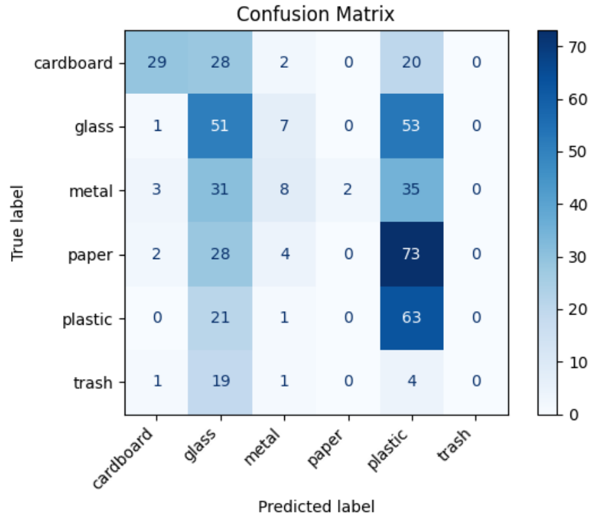
Figure 3: Confusion matrix for CNN
