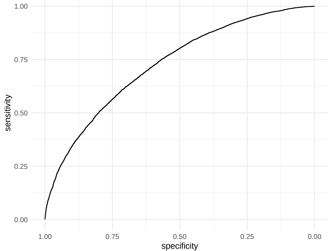
ROC (TRAIN) — AUC = 0.728
