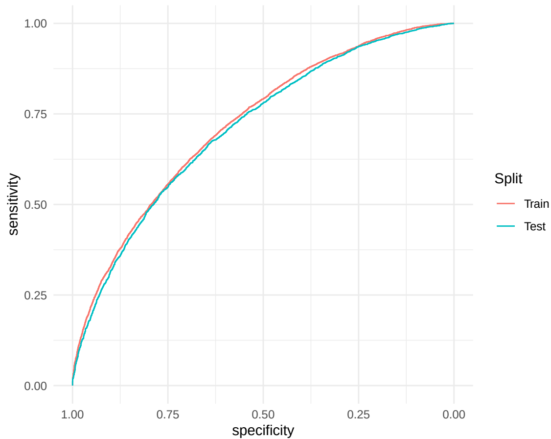
ROC – Train (0.723) vs. Test (0.713)
