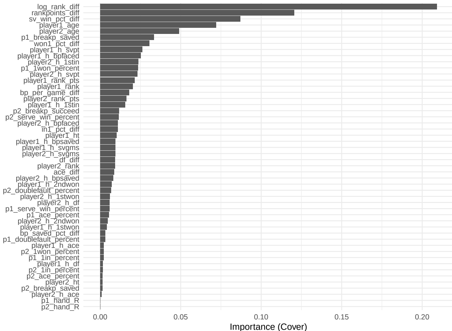
XGBoost Feature Importance (Cover)
