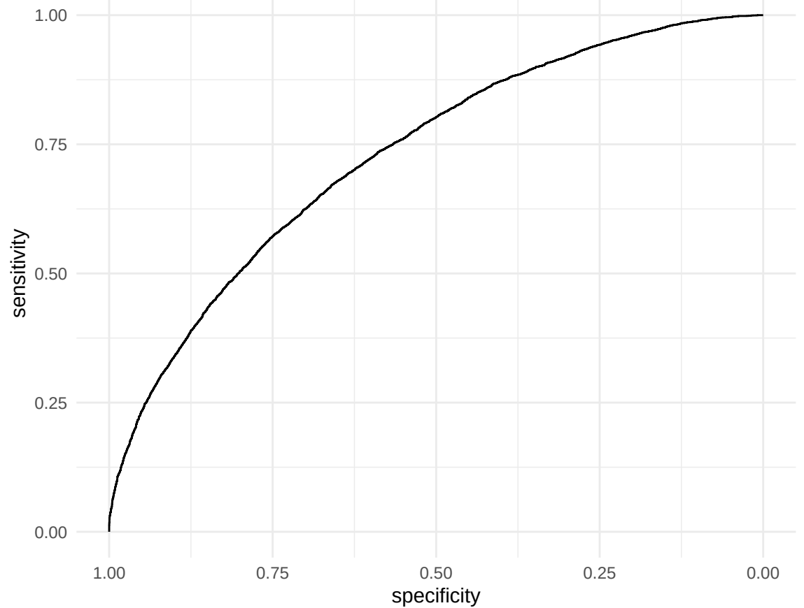
ROC RAW (TRAIN) – AUC = 0.730
