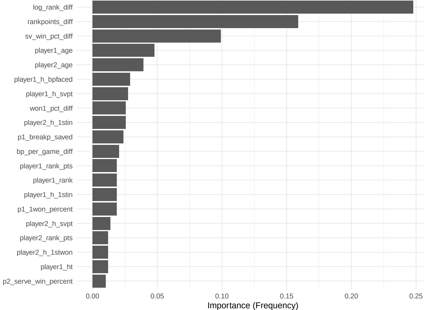
XGBoost Feature Importance (Frequency) – Top 20
