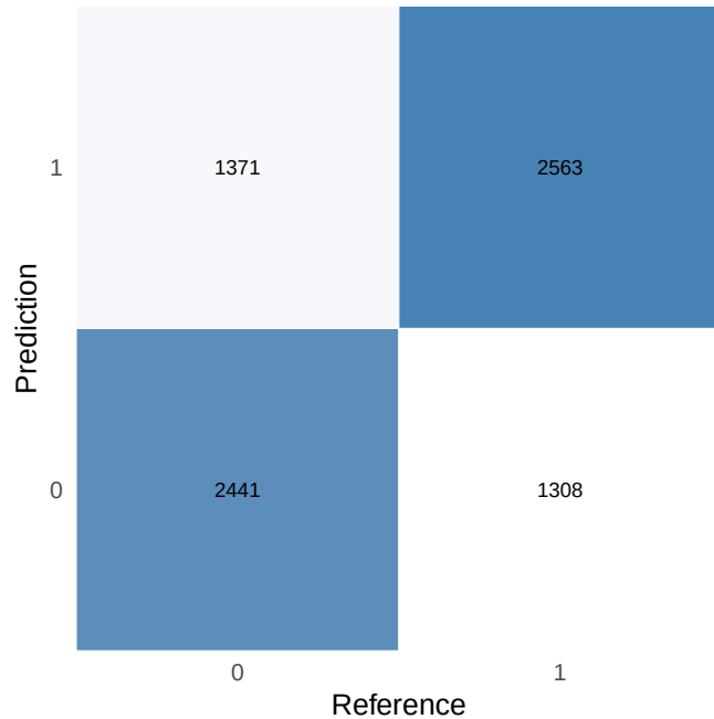
Random Forest (Test)
