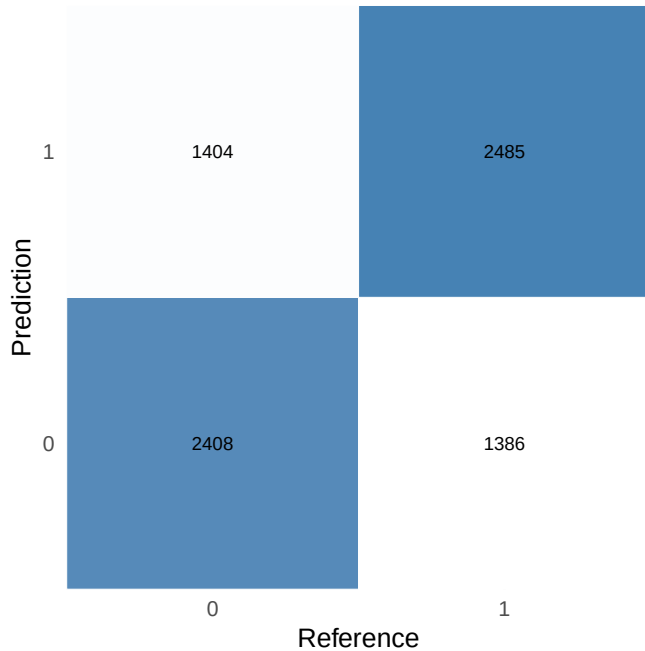
XGBoost (Test)
