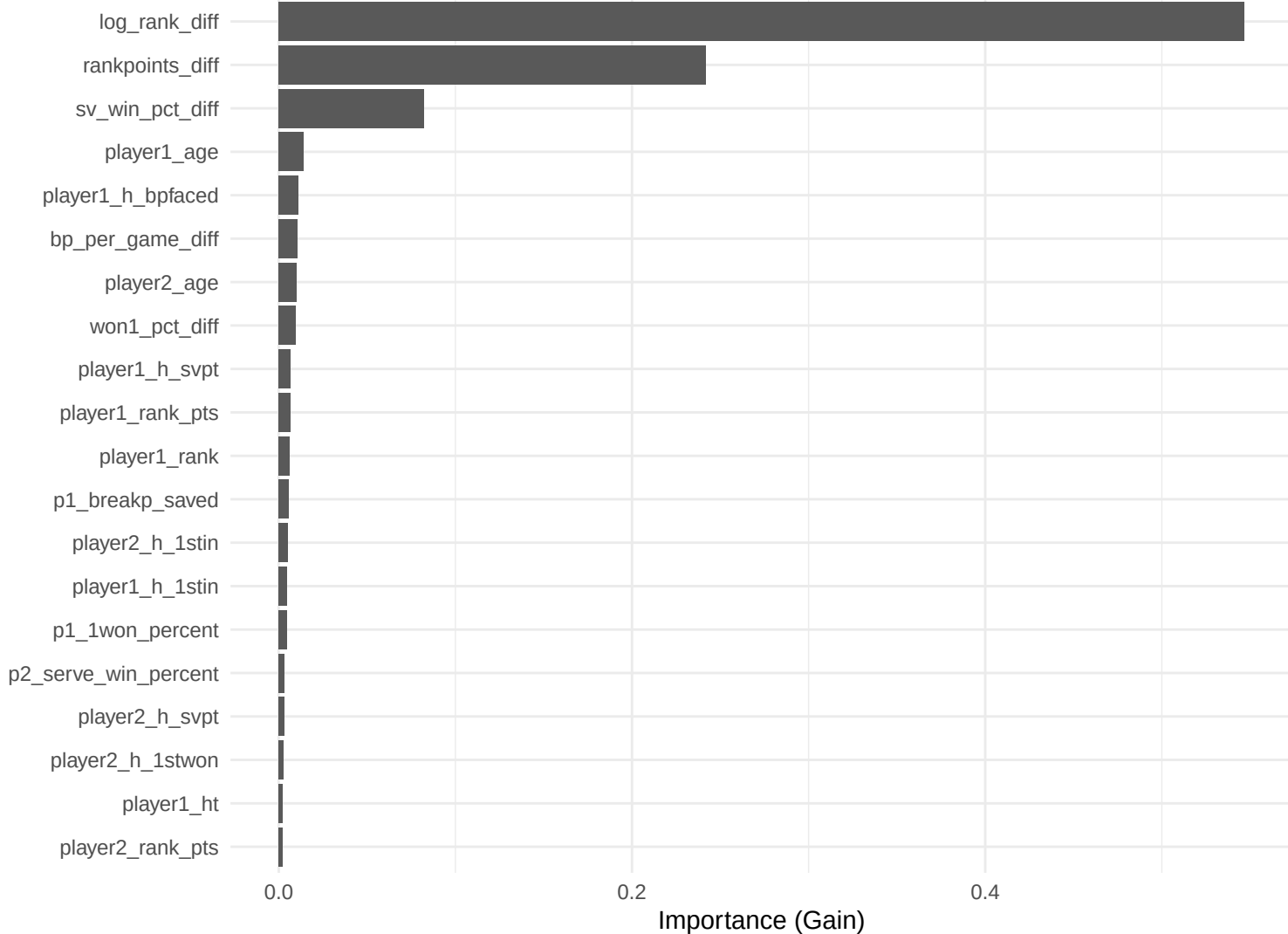
XGBoost Feature Importance (Gain) – Top 20
