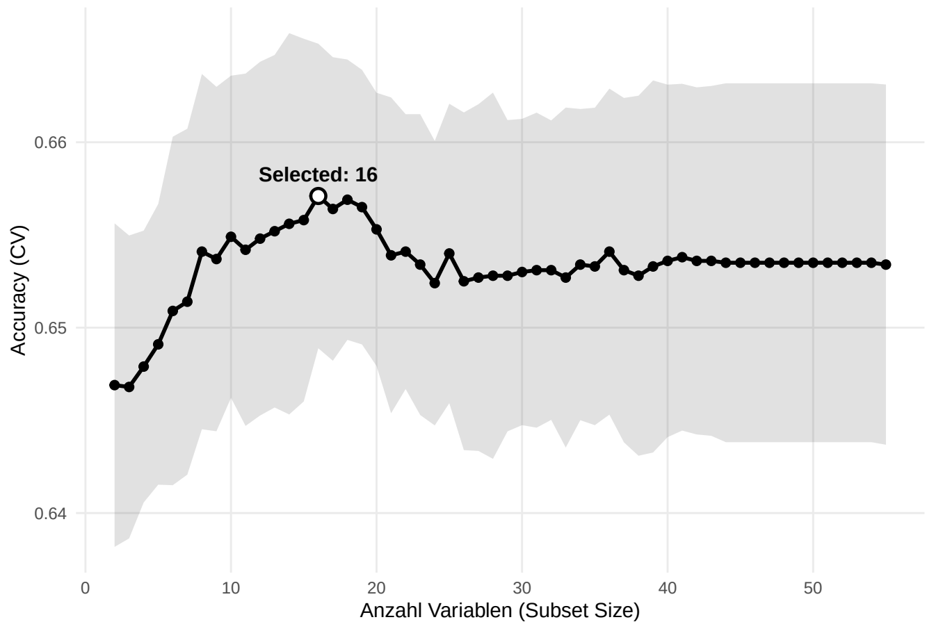
RFE Curve (Accuracy)
