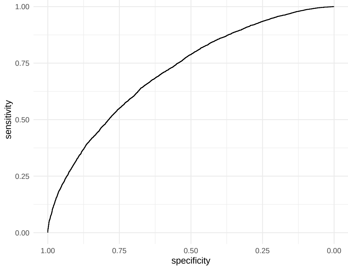
ROC (TRAIN) — AUC = 0.717
