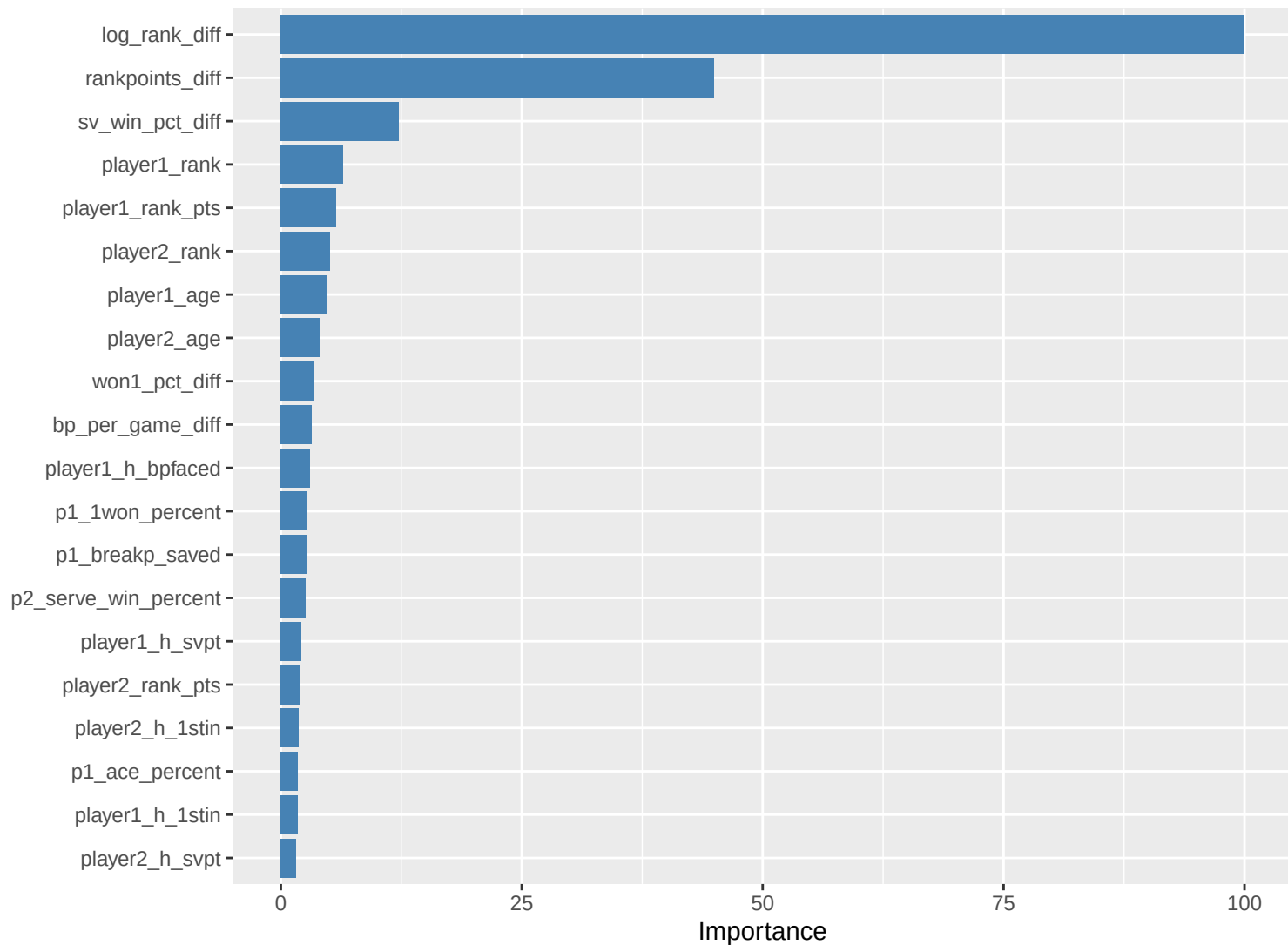
Top 20 Feature Importances (XGBoost)
