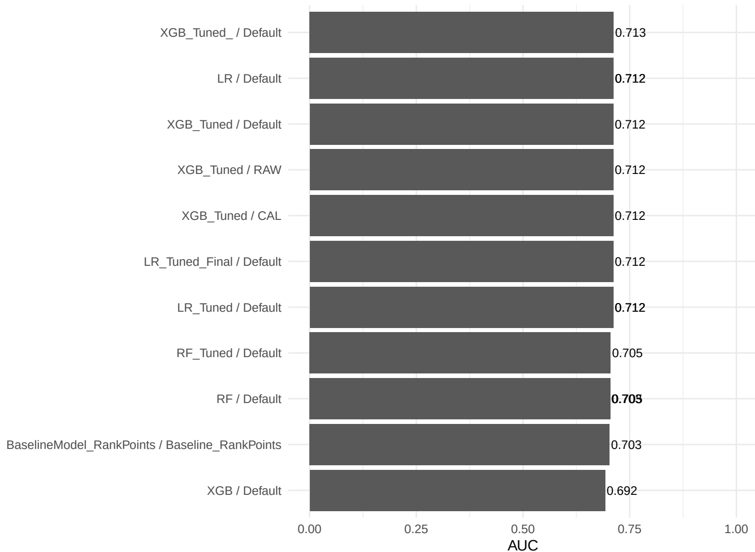
Model Comparison (TEST) – AUC
