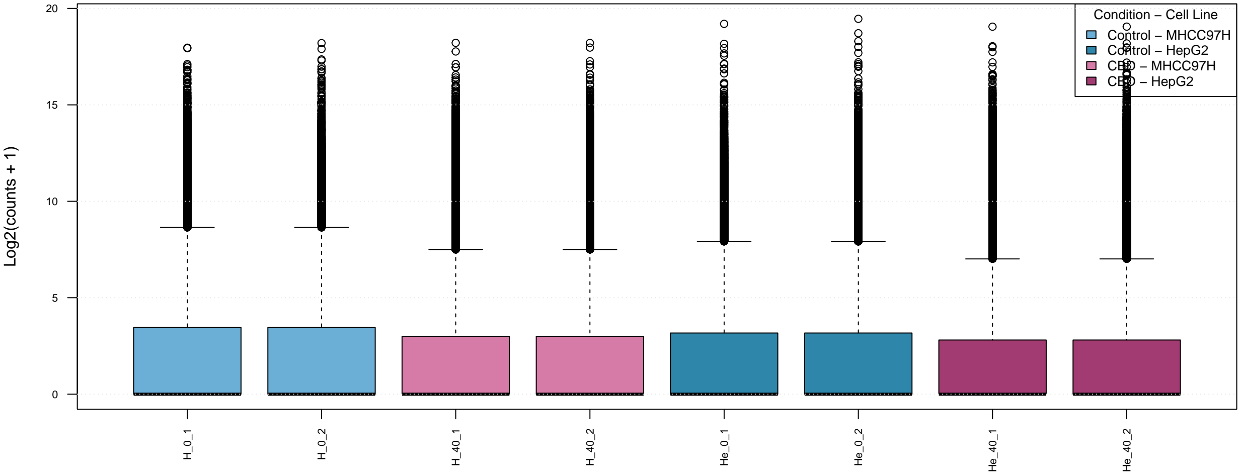
Raw counts distribution (log2) by Condition and Cell Line
