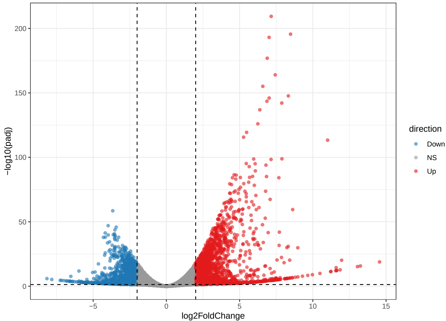
Volcano Plot – HepG2 (CBD vs Control)
