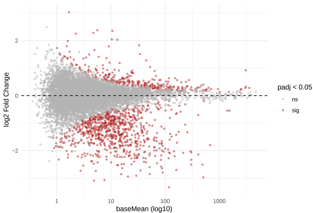
MA plot (TSV): CBD-THC vs DMSO
