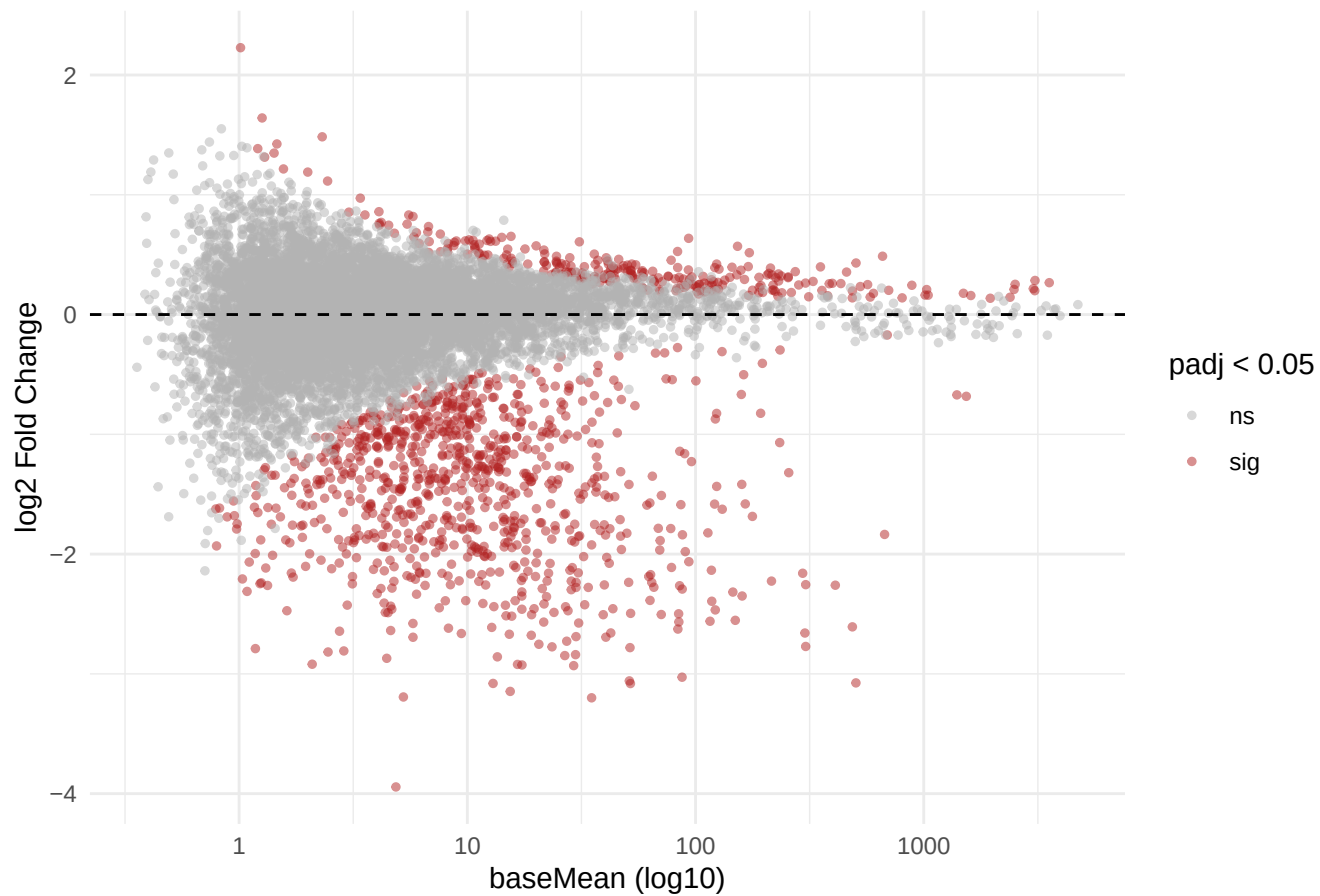
MA plot: DMSO–EtOH vs DMSO
