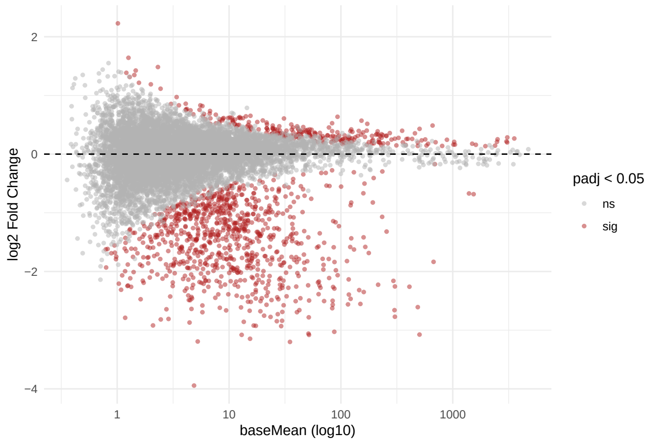
MA plot (TSV): DMSO-EtOH vs DMSO
