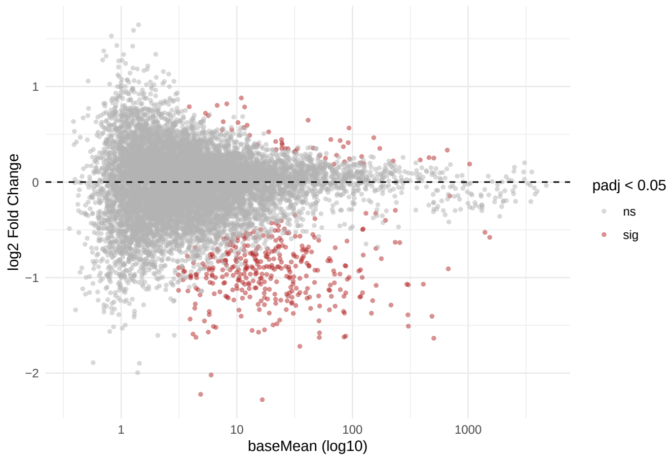
MA plot (TSV): EtOH vs DMSO
