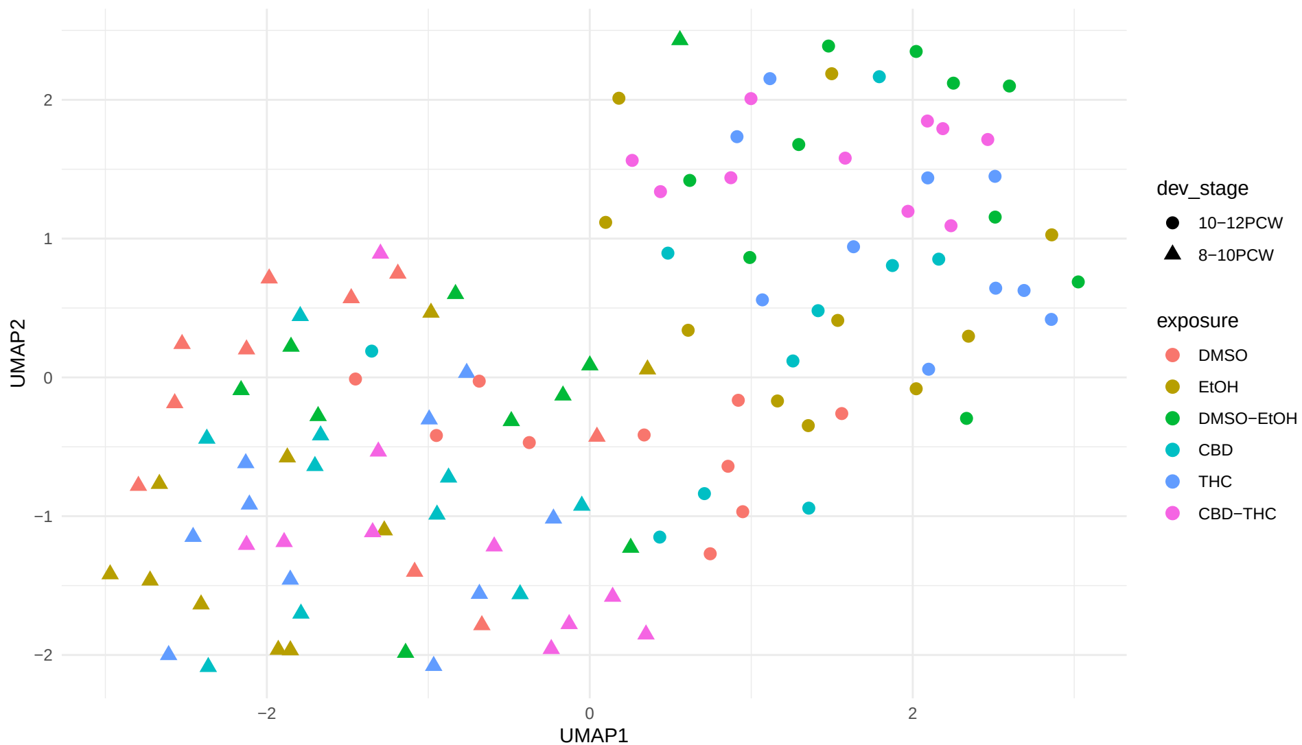
UMAP (logCPM, top 2000 genes)
