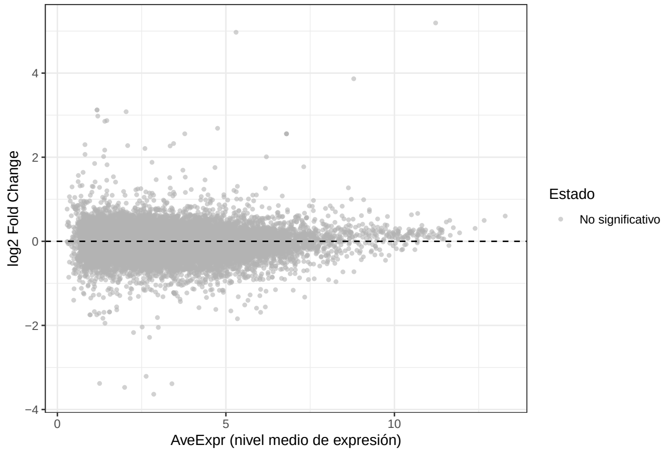
MA plot – CBD_vs_Mock
