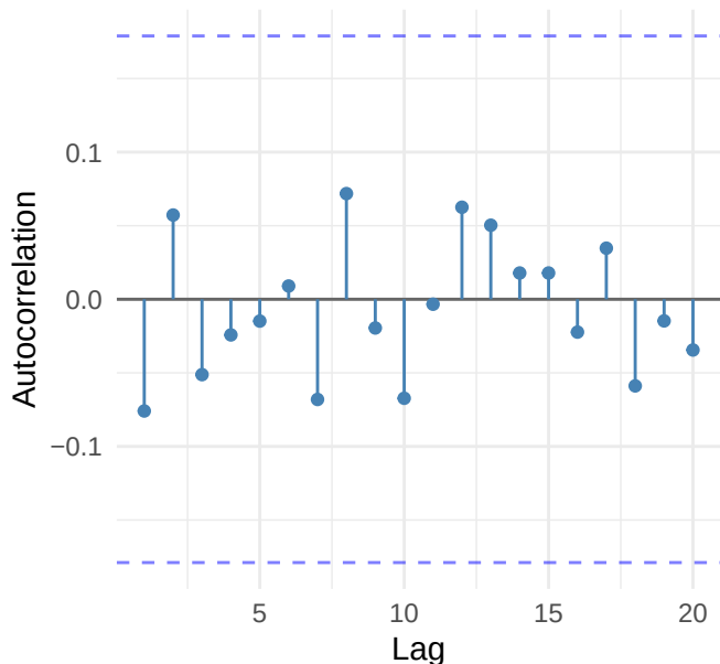
ACF of Residuals
