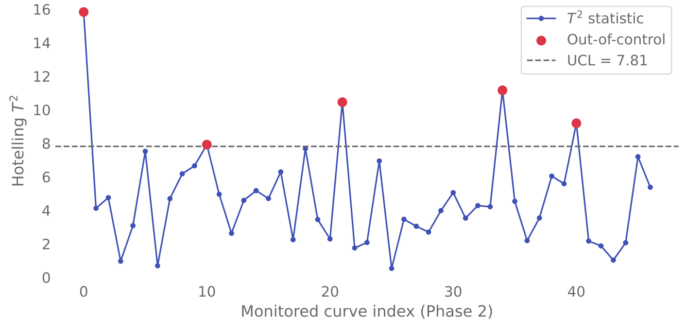
T^2 control chart: 5 alarm(s)
