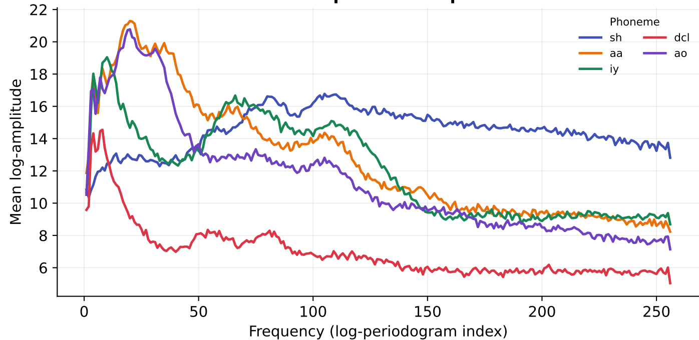
Class-mean spectra for 5 phonemes
