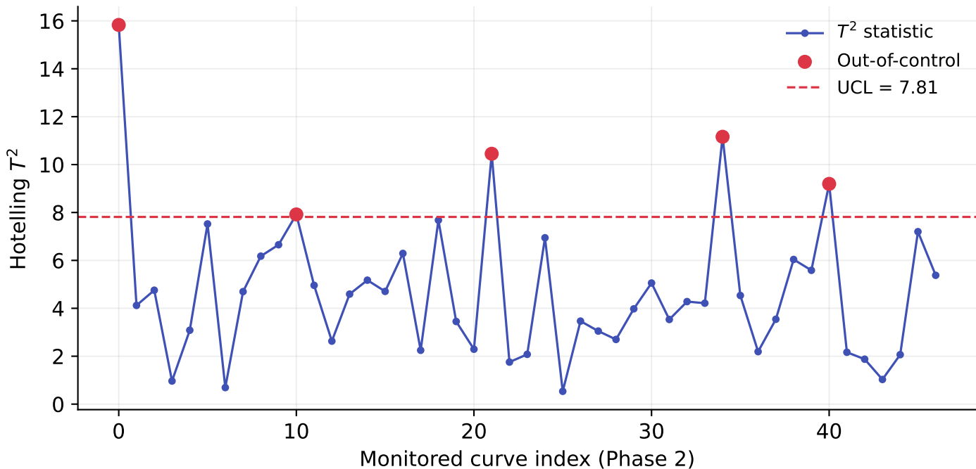
T^2 control chart: 5 alarm(s)
