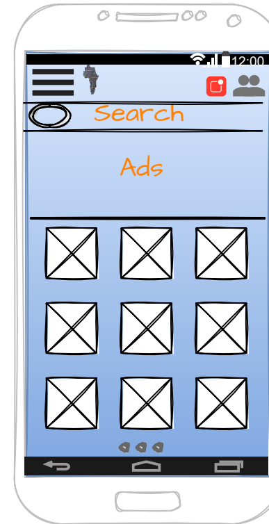
Main Screen
