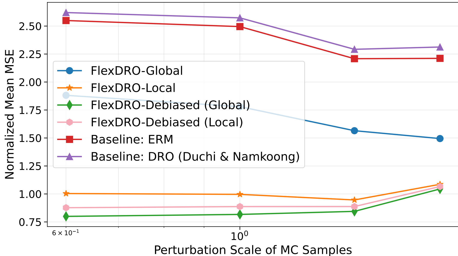
Mean MSE vs Perturbation Scale
