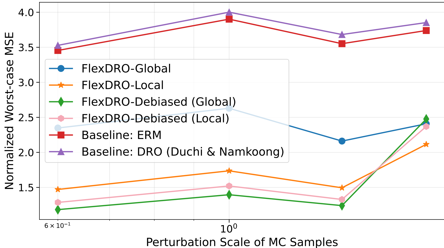
Worst-case MSE vs Perturbation Scale
