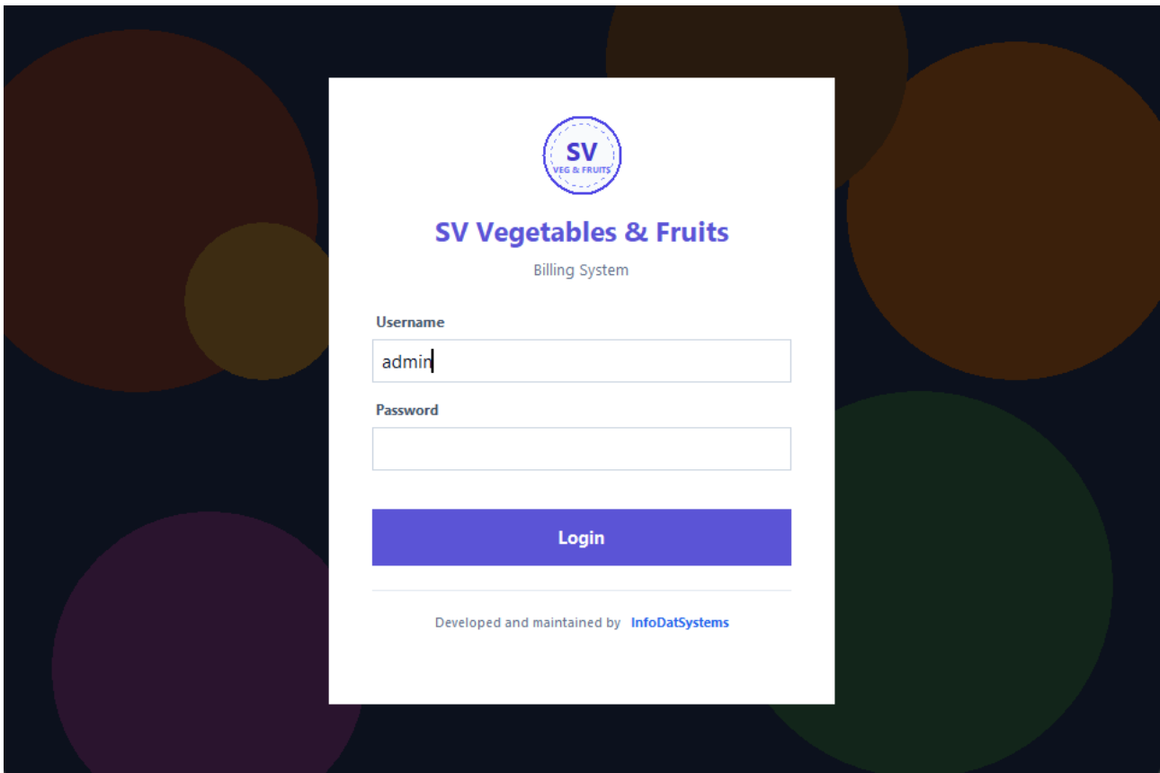
Sign-in screen
