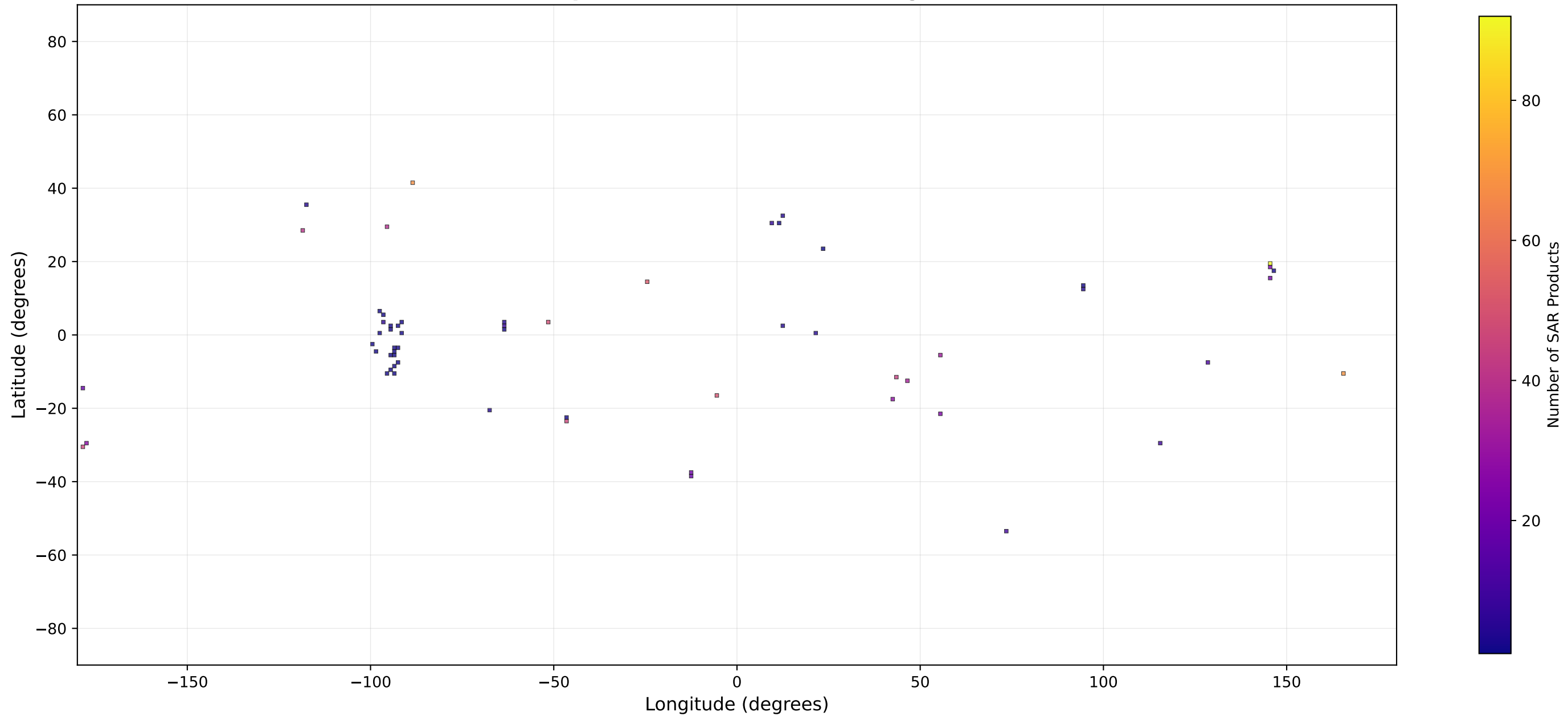
SAR Product Acquisitions World Map 967 products visualized on 1.0° grid
