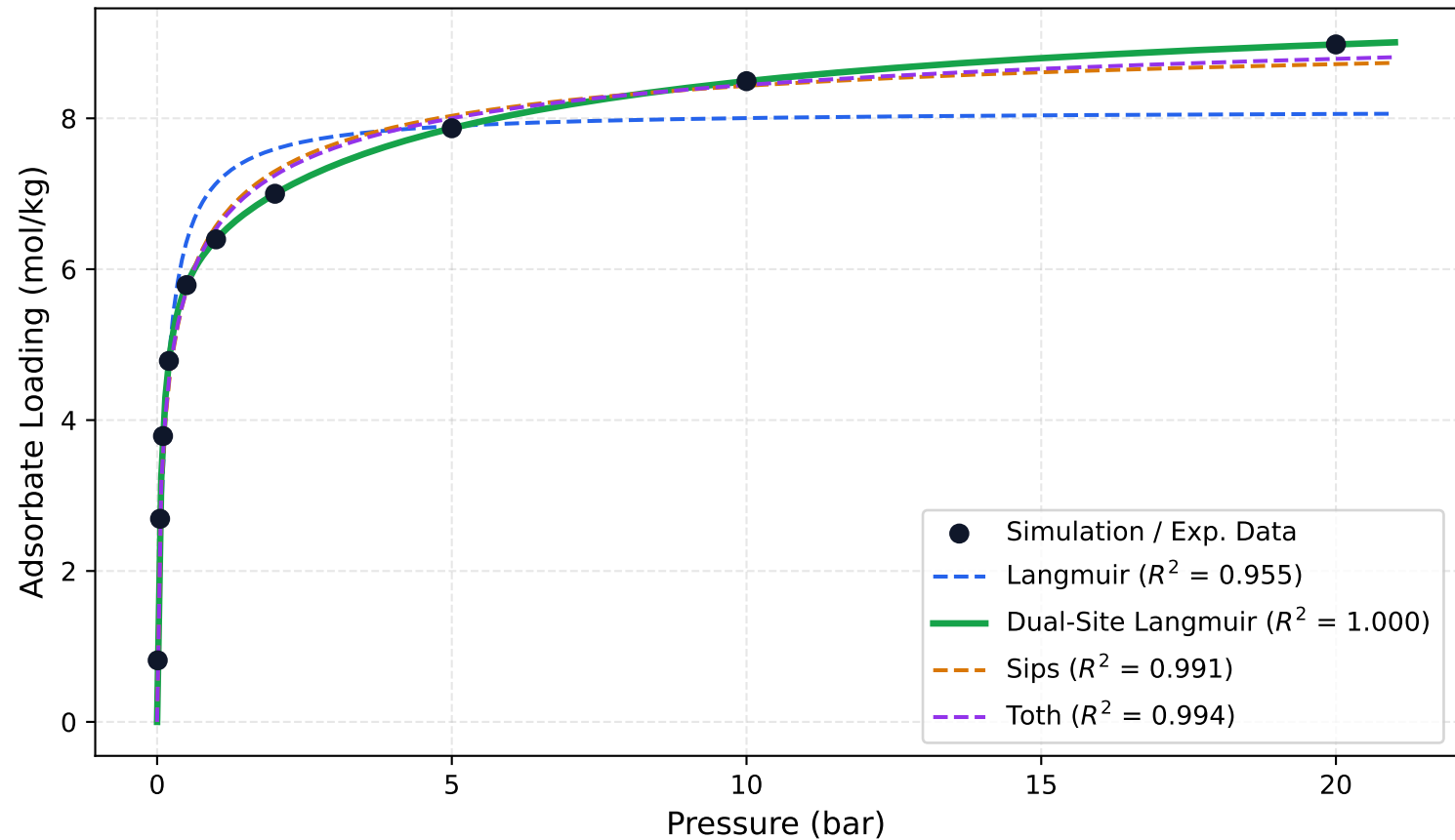
Adsorption Isotherm & Non-Linear Model Fits (CO 2 in Mg-MOF-74)
