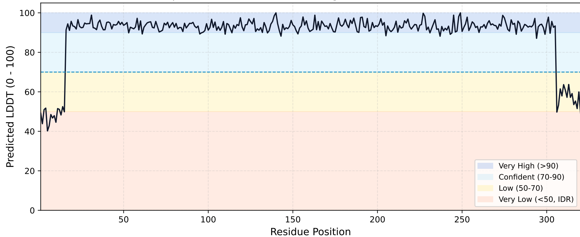
Per-Residue pLDDT Confidence Profile (Target Kinase Domain) — Mean: 89.6
