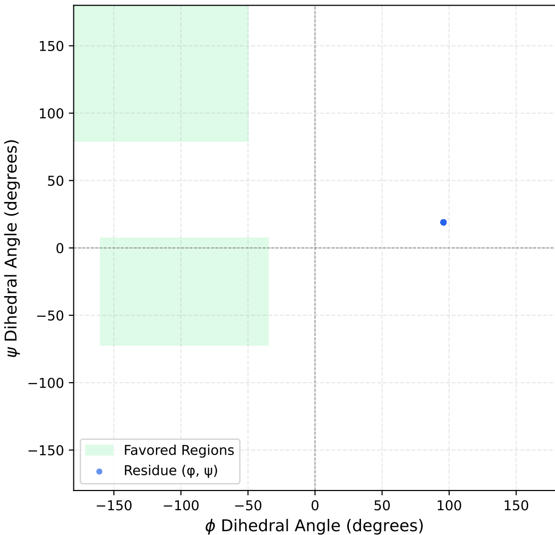
Ramachandran Plot (0.0% Favored)
